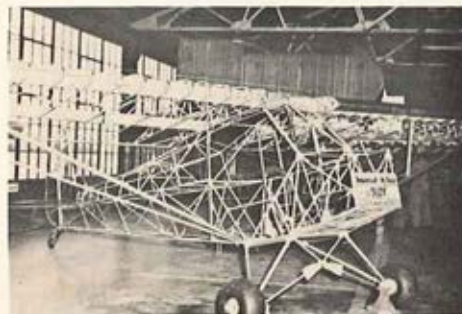
SUZY - The original "training aid"! Devoid of its fabric, the Piper L-4's basic tube steel framework and ultra-simple landing gear are shown in this '42 photo. Virtually maintenance-free, the Cub was liked by all.
